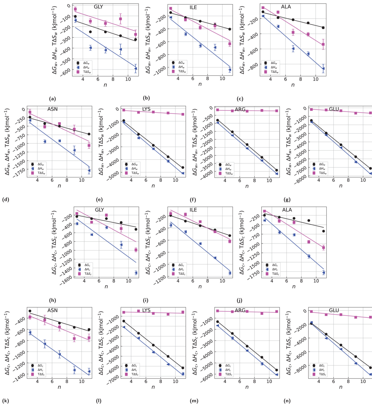
Fig. 8 Solvation free energy, enthalpy, and entropy ( \Delta G , \Delta H , T\Delta S ) changes with the polymer chain length n in \text{H}_2\text{O} and \text{C}_6\text{H}_{12} at 25^\circ\text{C} for each of the polypeptides considered in this work (GLY, ALA, ILE, ASN, LYS, ARG, GLU). The continuous lines connecting the points show the representative linear fitting. The data representing the hydration thermodynamics in \text{H}_2\text{O} are shown from (a) to (g), whilst those corresponding to \text{C}_6\text{H}_{12} are plotted from (h) to (n) for each of the polypeptides. Negative \Delta G and \Delta H represent an energetic gain upon solvation, whereas a negative T\Delta S represents an entropic loss, upon solvation.
