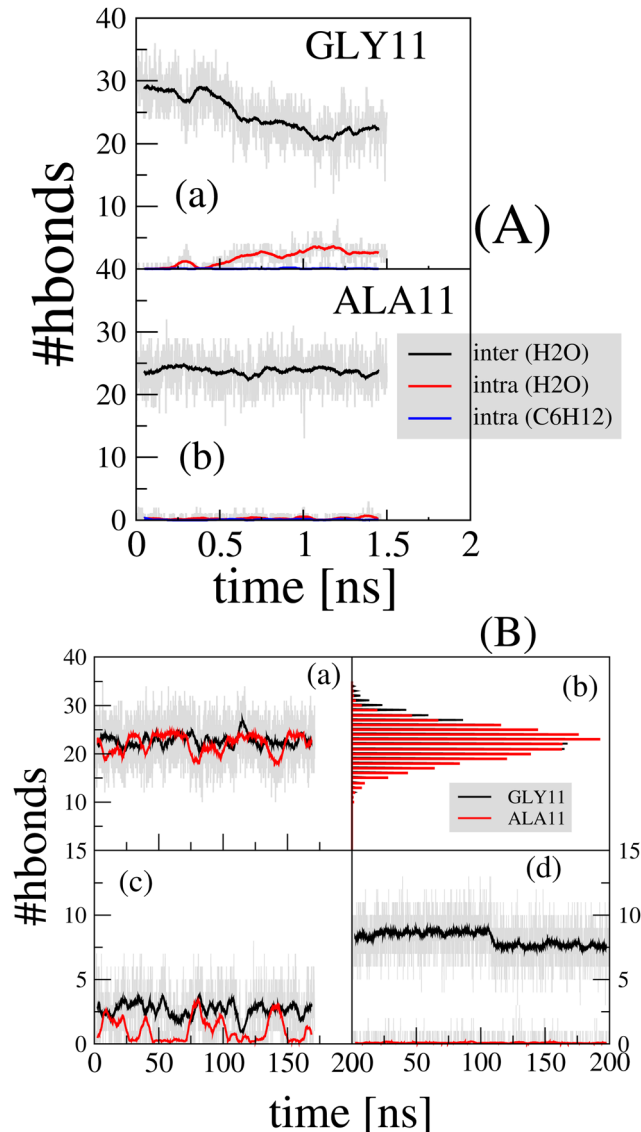
Fig. 4 Top panel (A): Initial stage evolution of the number of hydrogen bonds for GLY11 ((A)-(a)) and ALA11 ((A)-(b)). Both inter- ( \text{H}_2\text{O} –solute black line, (A)-(a) & (A)-(b)) and intra- (solute–solute in \text{H}_2\text{O} red line and \text{cC}_6\text{H}_{12} blue line, (A)-(a) & (A)-(b)) molecular hydrogen bonds are plotted. Bottom panel (B): Long time evolution of the number of hydrogen bonds of GLY11 (black line) and ALA11 (red line). (B)-(a) Solute– \text{H}_2\text{O} hydrogen bonds; (B)-(b) histogram distribution of (B)-(a); (B)-(c) solute–solute hydrogen bonds in \text{H}_2\text{O} ; (B)-(d) solute–solute hydrogen bonds in \text{cC}_6\text{H}_{12} .
